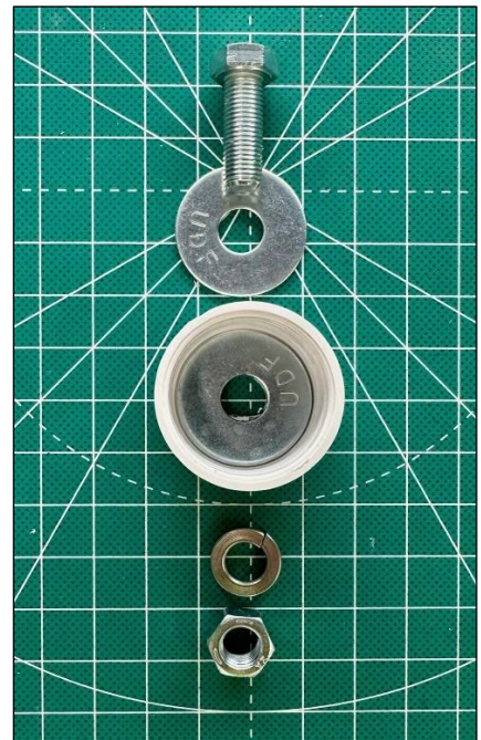
Drill a 3/8" hole in the center of end cap. Use 3/8"-24 hardware including 2 fender washers on both sides of the PVC end cap.
