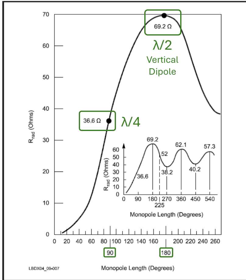
Fig 9-7—Radiation resistances ( R_{\text{rad(l)}} , at the current maximum) of monopoles with sinusoidal current distribution. The chart can also be used for dipoles, but all values must be doubled.
